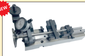
Valve concentricity device (unique linear guideways design)
